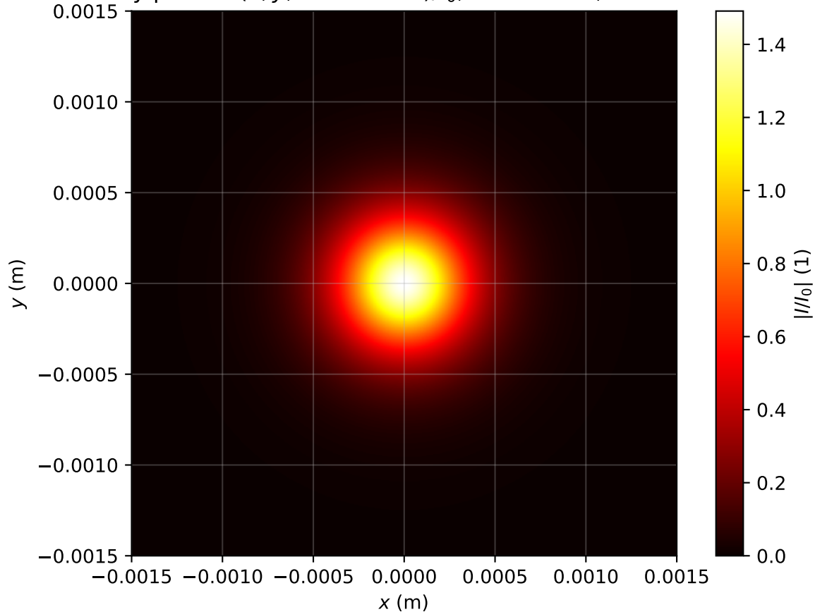
Intensity profile I(x, y, z = 3.503m)/I_0 , Pin=0.9Pcr, artificial time
